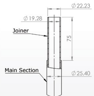
Mast Top Section Detail
